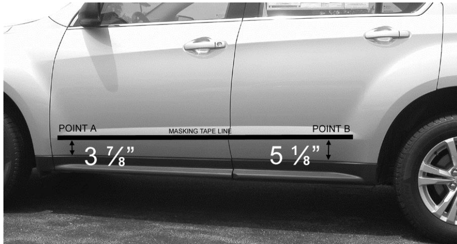
Measure up from the top of black cladding
